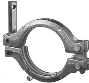
SCREW CLAMP COUPLING 6"
